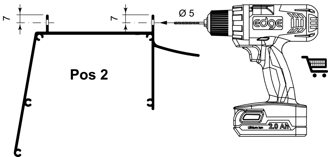
Detail Post fixing
