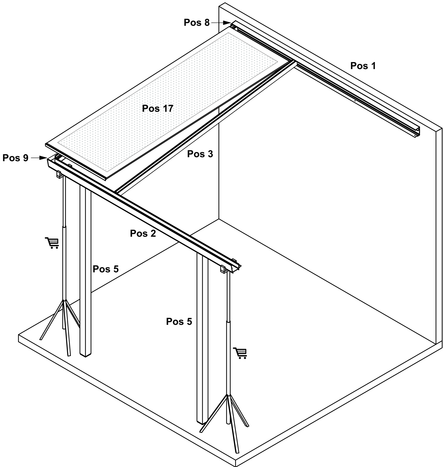
Detail assembling Support to the Wall profile
