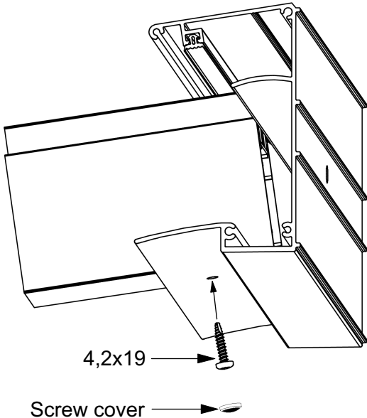
Detail assembling Support to the Wall profile
