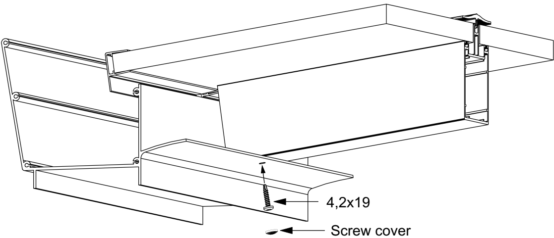
Detail assembling Support to the Gutter
